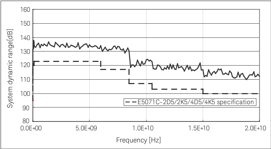
Figure 2. System dynamic range (specification and actual measurement data example, IF bandwidth 10 Hz)
