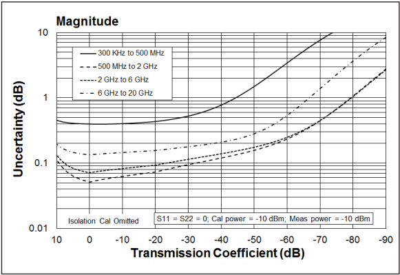
Transmission uncertainty (specification)
