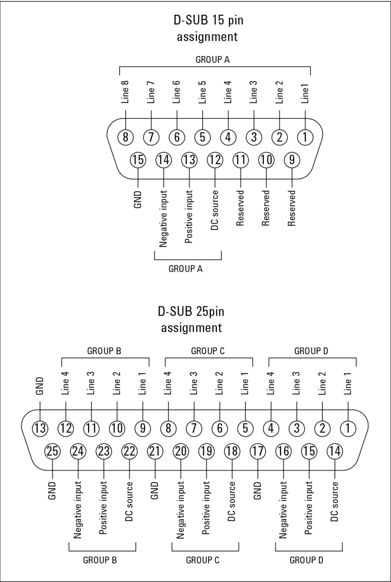
Figure 16. Control line pin assignment (E5092A-020)
