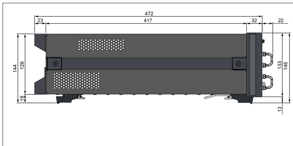
Figure 13. Dimensions (side view, with Option E5092A-020, in millimeters, nominal)
