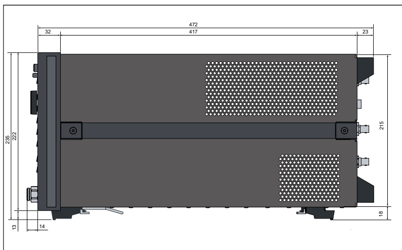
Figure 9. Dimensions (side view, E5071C with Option 2D5/2K5/4D5/4K5, in millimeters)
