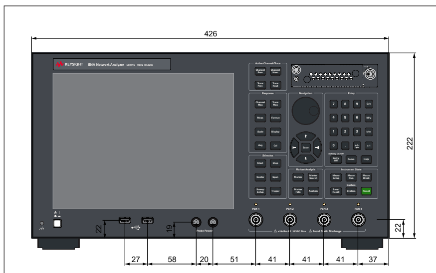
Figure 4. Dimensions (front view, E5071C with Option 430/435/440/445/460/465/480/485, in millimeters)
