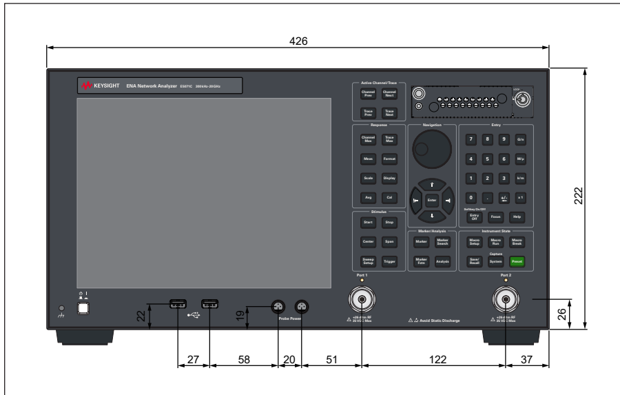
Figure 5. Dimensions (front view, E5071C with Option 2D5/2K5, in millimeters)
