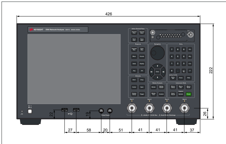
Figure 6. Dimensions (front view, E5071C with Option 4D5/4K5, in millimeters)
