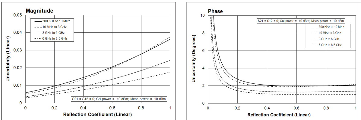
Reflection uncertainty (specification)
