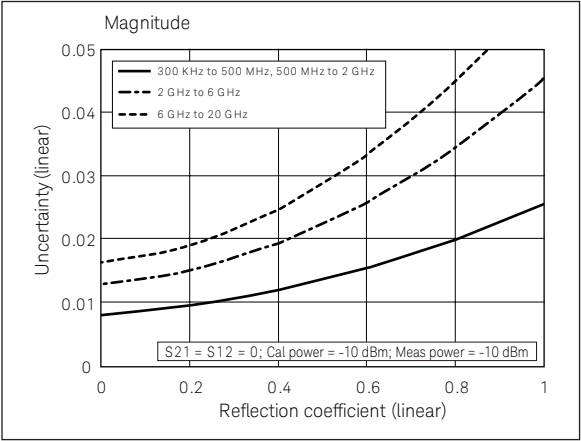
Reflection uncertainty (specification)
