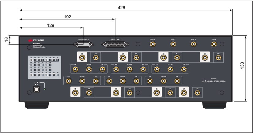
Figure 10. Dimensions (front view, with Option E5092A-020, in millimeters, nominal)
