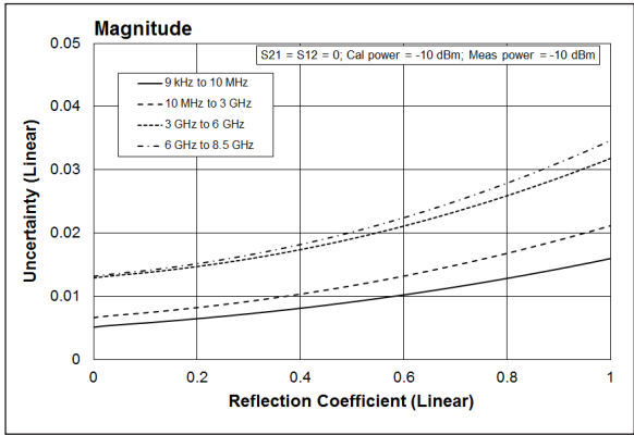
Reflection uncertainty (specification)
