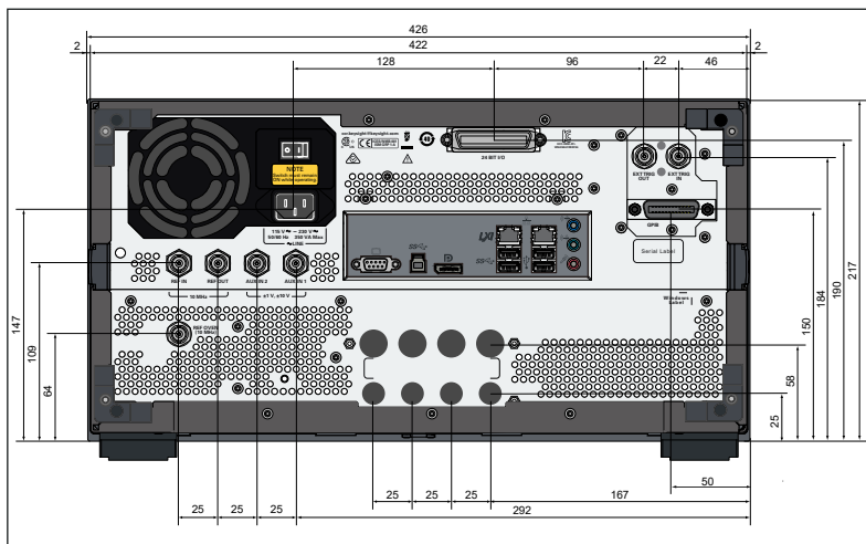
Figure 7. Dimensions (rear view with Option 1E5, in millimeters)
