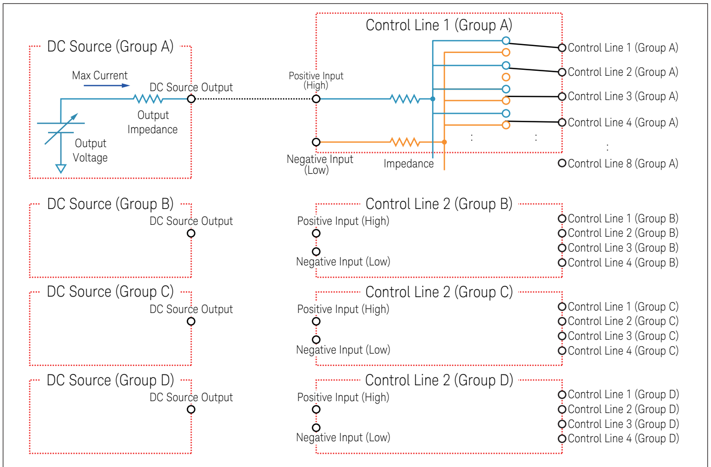
Figure 15. DC control line (E5092A-020)
