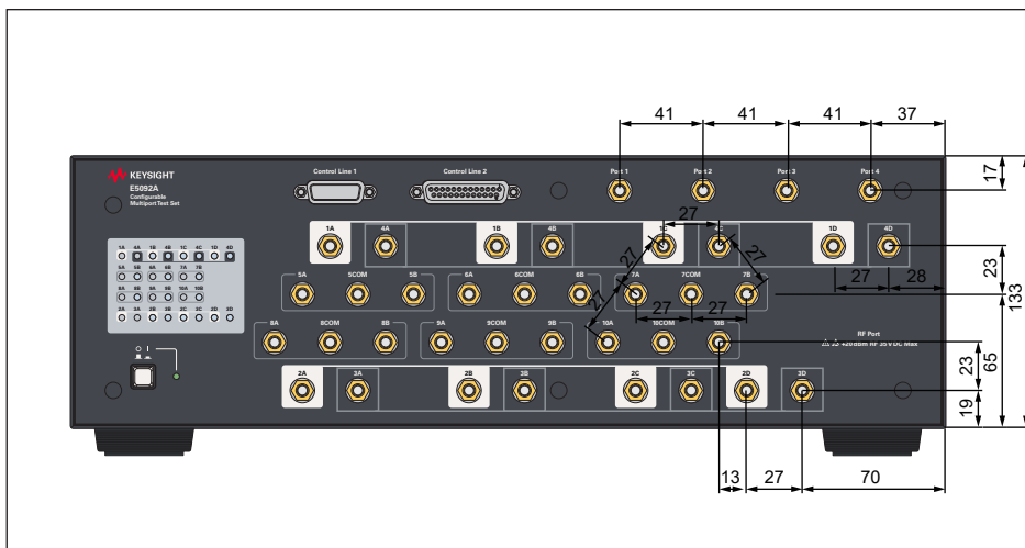
Figure 11. Dimensions (pitch between switches, with Option E5092A-020, in millimeters, nominal)
