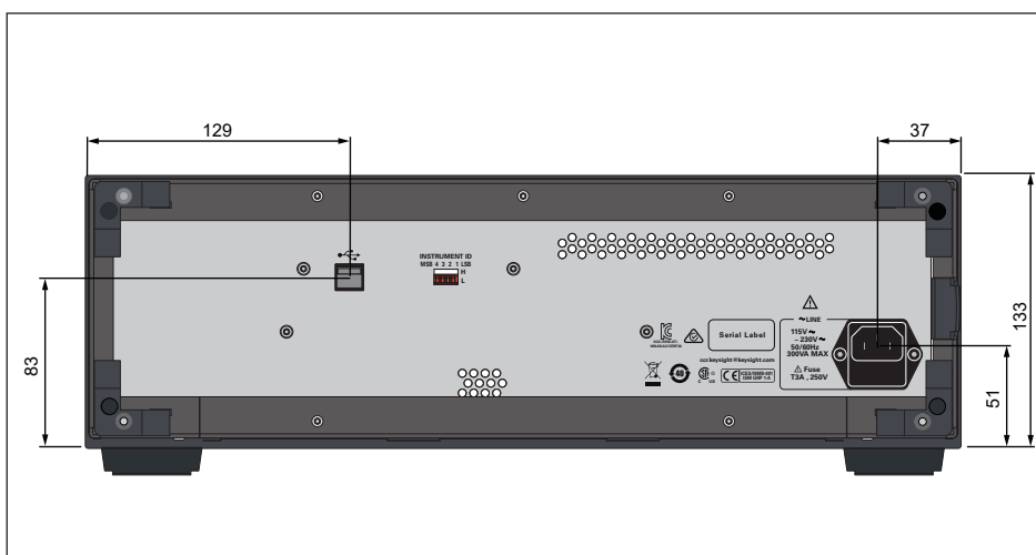
Figure 12. Dimensions (rear view, with Option E5092A-020, in millimeters, nominal)
