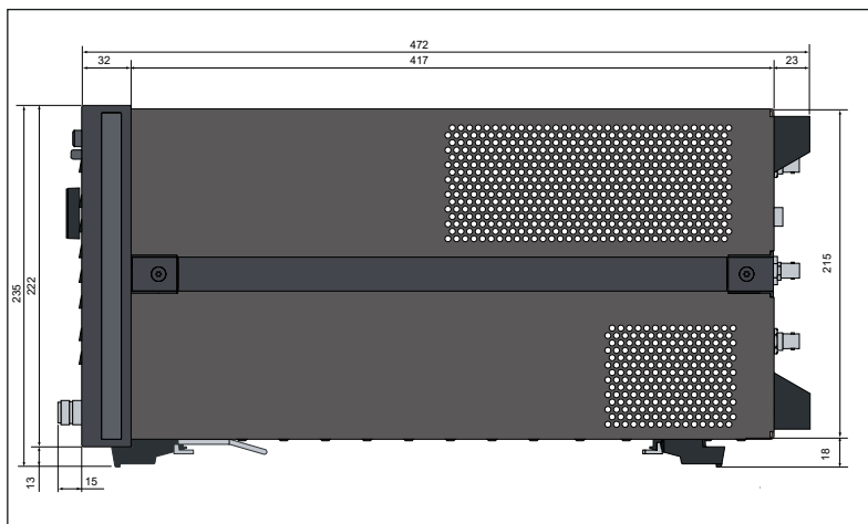
Figure 8. Dimensions (side view, E5071C Option 230/235/240/245/260/265/280/285/430/435/440/445/460/ 465/480/485, in millimeters)
