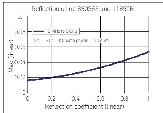
Reflection uncertainty 10 MHz to 3 GHz (typical) Magnitude
